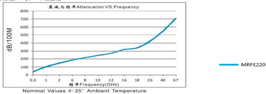
衰减vs. 频率 Attenuation vs. Frequency (dB/100m)
