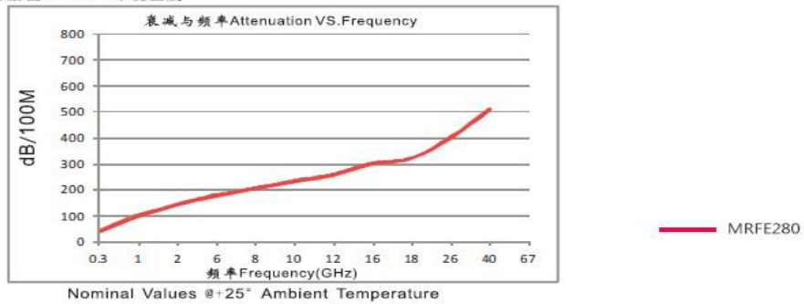
衰减vs. 频率 Attenuation vs. Frequency (dB/100m)
